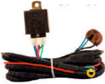
H L WIRING KIT A4 BAKELITE BULB HOLDER - DIRECT EARTHING WITH 80 AMP. RELAY RAI - 1883
