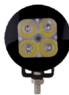
UNIVERSAL SMALL SPOT LENS (12V / 24V WITH OSRAM LED) RAI - 1570D / 1570AD
